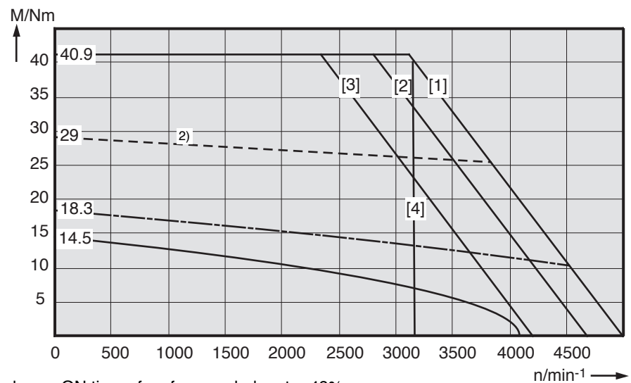
Fig 6.7: Torque-speed characteristics MAC 093
