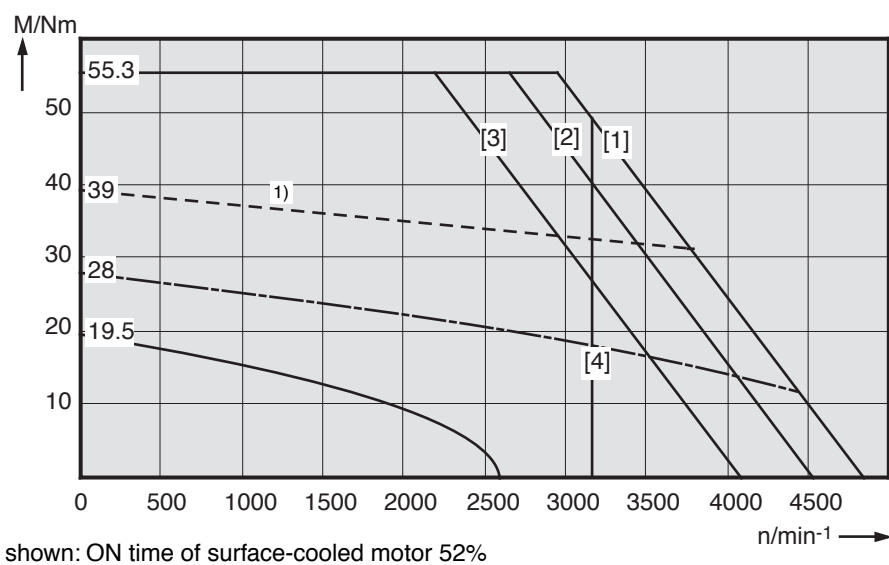
Fig 6.9: Torque-speed characteristics MAC 093
