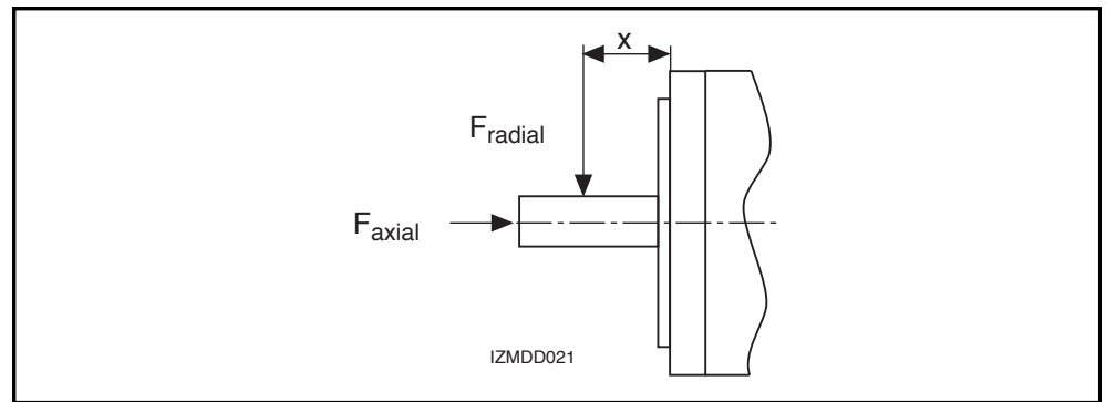
Fig 4.11: Shaft load
