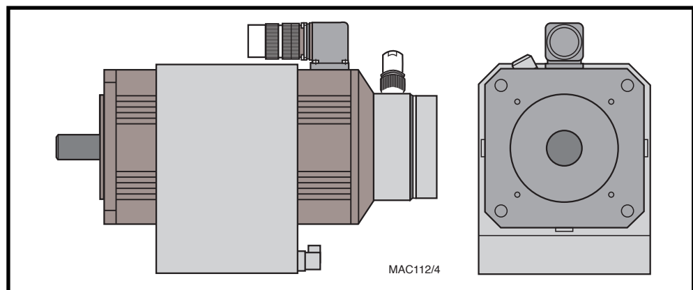
Fig 2.10: An example of a MAC servo motor with radial surface cooling with the blower under the motor shaft
